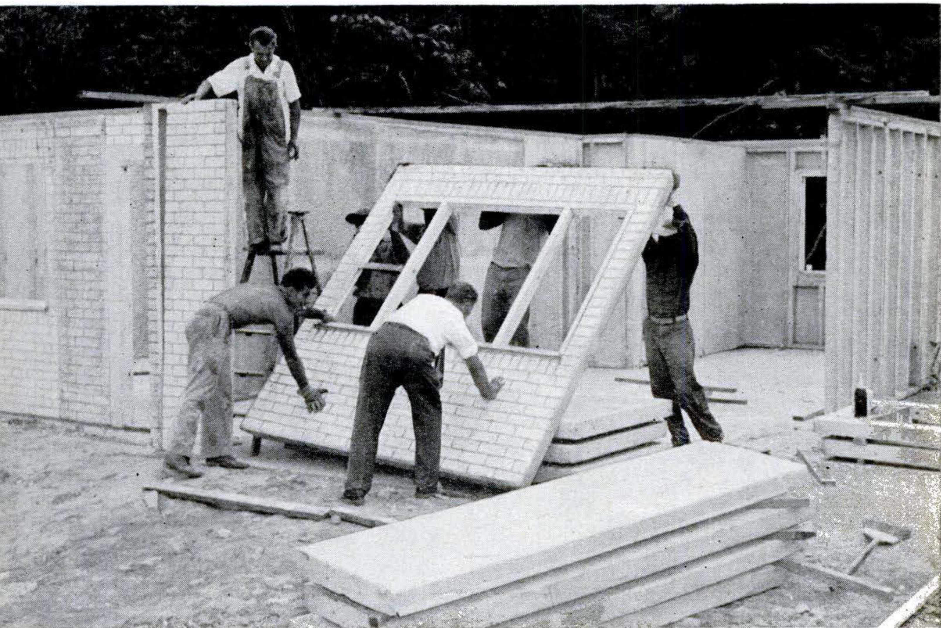
PICTURE-WINDOW PANEL is raised. Carpenter (on ladder) waits to nail down plate. Panels are available with openings for three sizes
